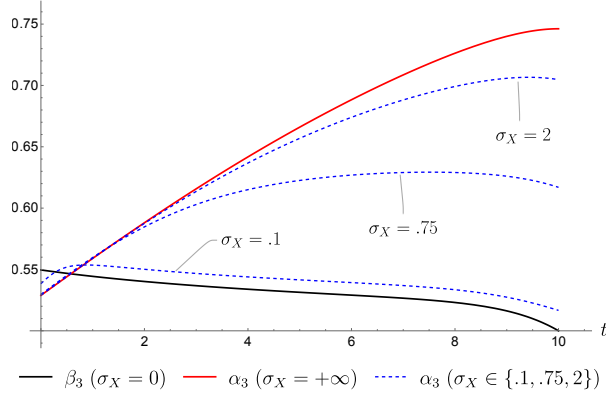
Figure 3: Sender’s signaling coefficient as \sigma_X varies. Other parameters: (k, \gamma^o, r, \sigma_Y) = (1, 1, 1, 1.5)
